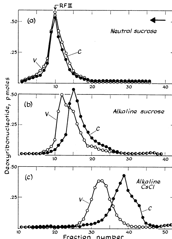
FIG. 2. Characterization of RF synthesized in vitro . Triphosphate mixture (40 \mu l with [^3\text{H}]\text{TTP} , 2900 cpm/pmol), ^{32} P-labeled M13 SS (10 \mu l, 260 pmol, 1280 cpm/pmol), and fraction A (200 \mu l) were incubated at 37° for 5 min. Sodium dodecyl sulfate was added (25 \mu l, 5%), and the RF was purified by sucrose gradient centrifugation and ethanol precipitation (1). 51 pmol of ^{32} P-labeled viral DNA, V, and 53 pmol of ^3\text{H} -labeled complementary DNA, C, were recovered as RF. (a) Centrifugation of product DNA (5 pmol) for 4.5 hr at 4° through a neutral sucrose gradient [5–20% in 1.0 M NaCl, 1.0 mM EDTA, and 10 mM Tris·HCl (pH 8.0) in an SW56 rotor]. (b) Centrifugation of product DNA (5 pmol) for 4.5 hr at 4° through an alkaline sucrose gradient (5–20% in 0.8 M NaCl, 0.2 M NaOH, 1 mM EDTA in an SW 56 rotor). (c) Equilibrium alkaline CsCl sedimentation of product DNA (5 pmol) as described by Ray (12).
